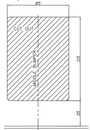
UNDERSIDE BUMPER
